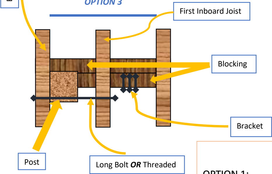
POST AT END JOIST – OPTION 3
