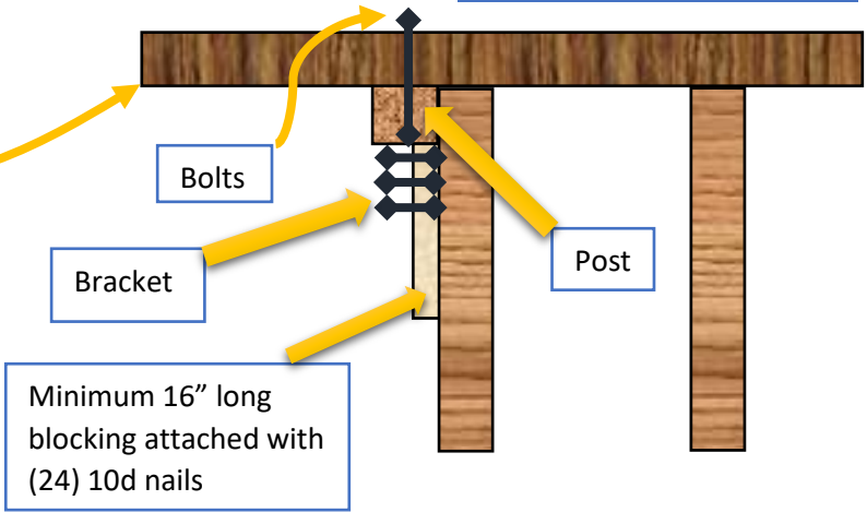
POST ALONGSIDE JOIST – OPTION 2
