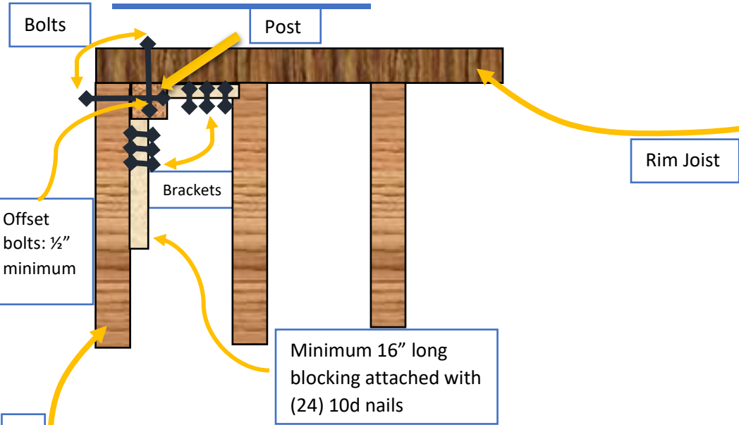
POST AT OUTSIDE CORNER – OPTION 1
